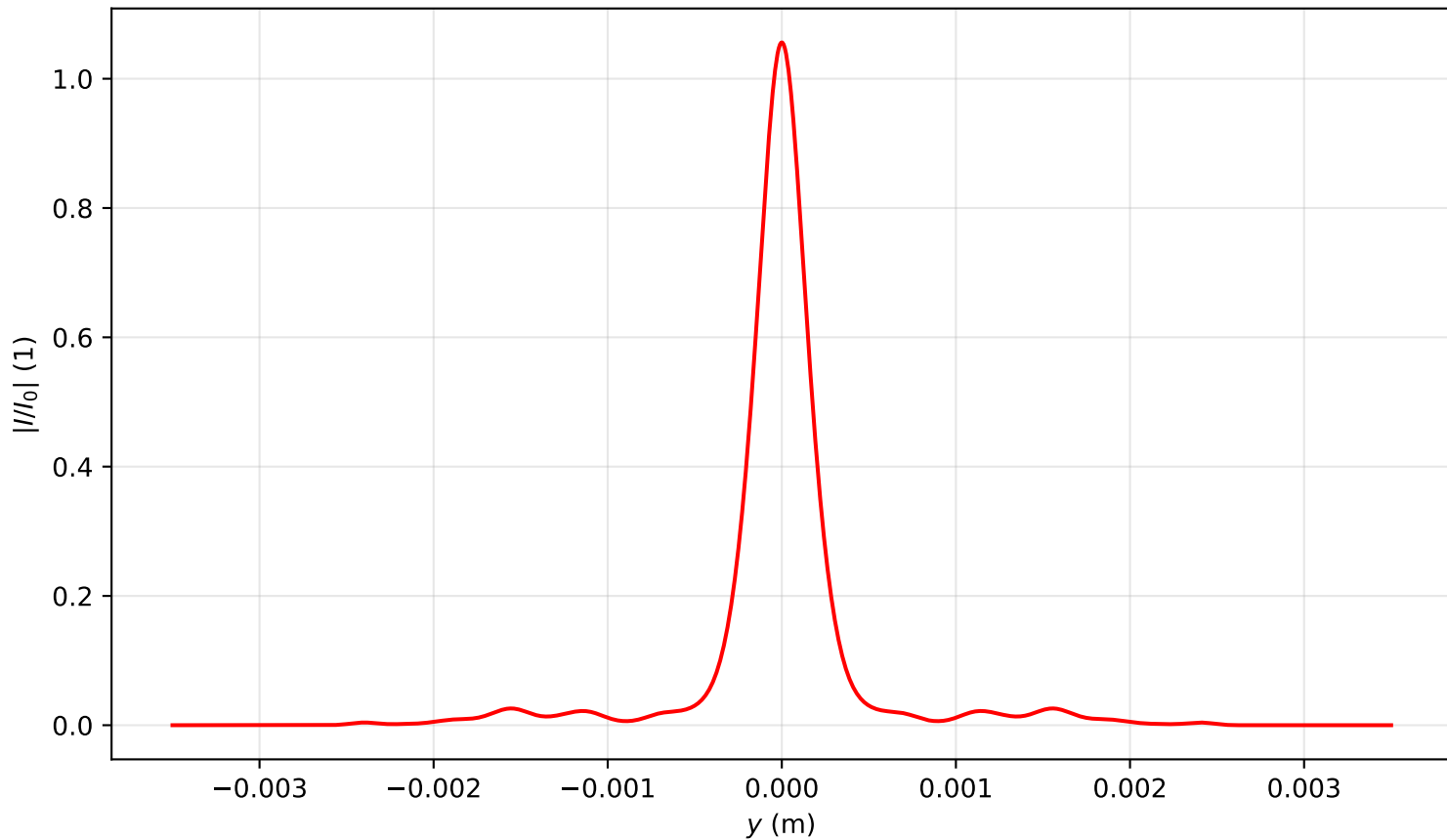
Intensity profile I(x=0, y, z=3.821)/I_0 , P_{in}=4.5P_{cr} , artificial time
